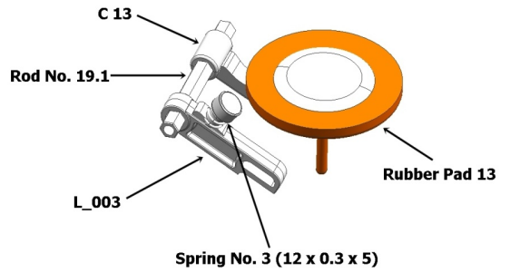
Cover 13
