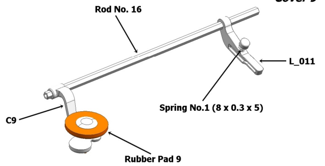
Cover 9
